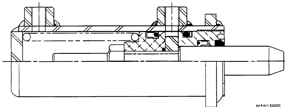
Brake Cylinder Internal Components
